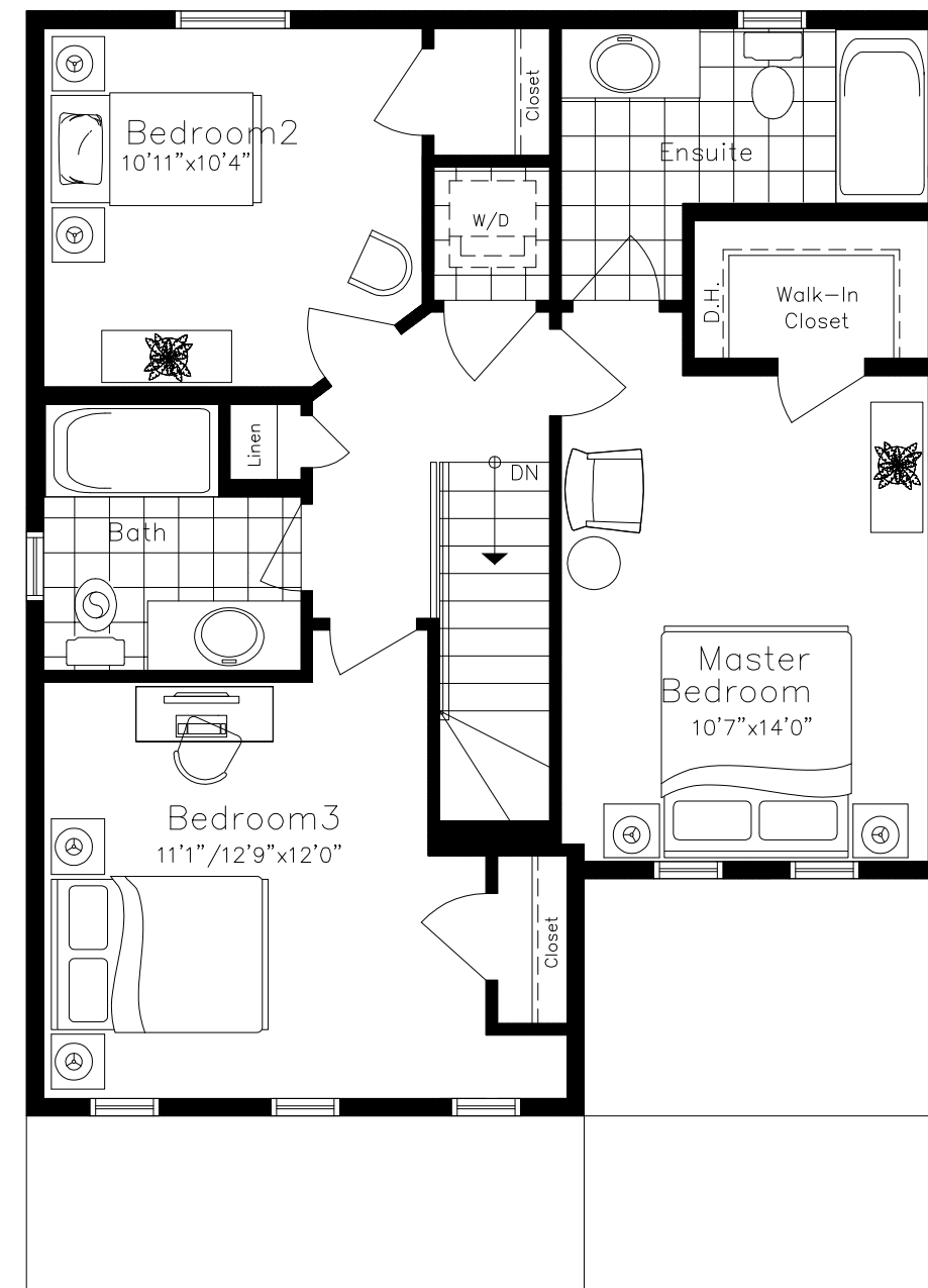
SECOND FLOOR PLAN - 772 SQ.FT. ELEV. C
