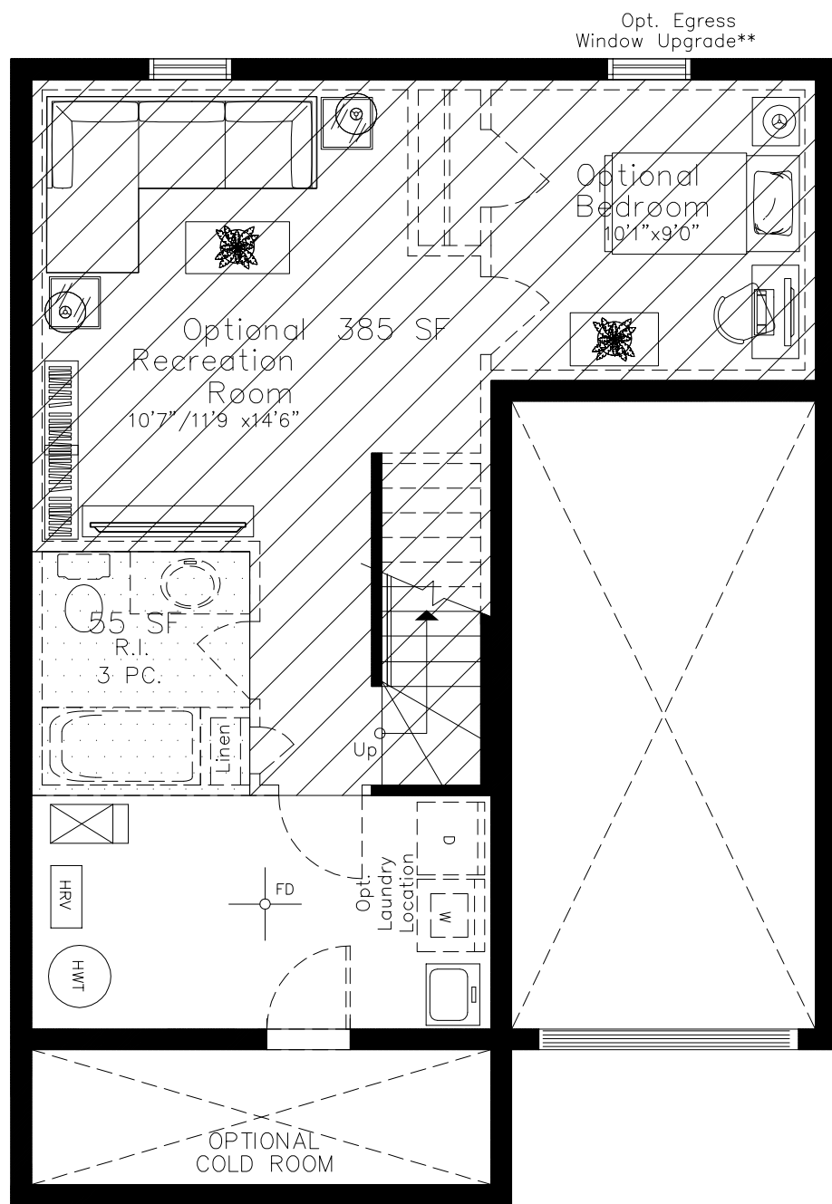
BASEMENT PLAN ELEV. C
