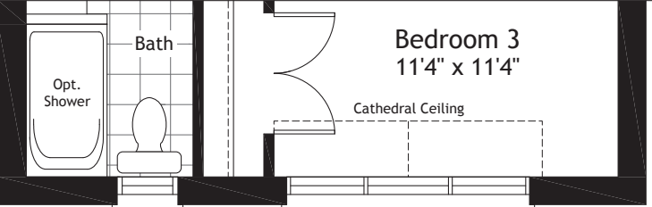
Loft Plan Elev. C
