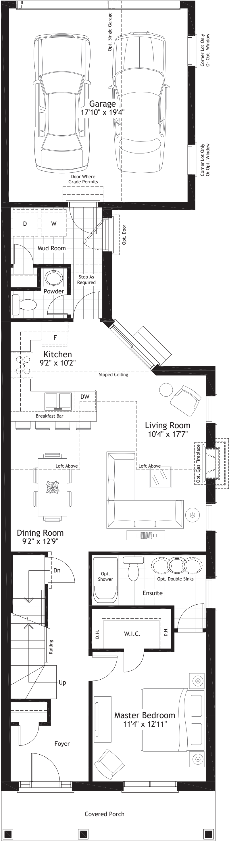
Main Floor - Elev. C
