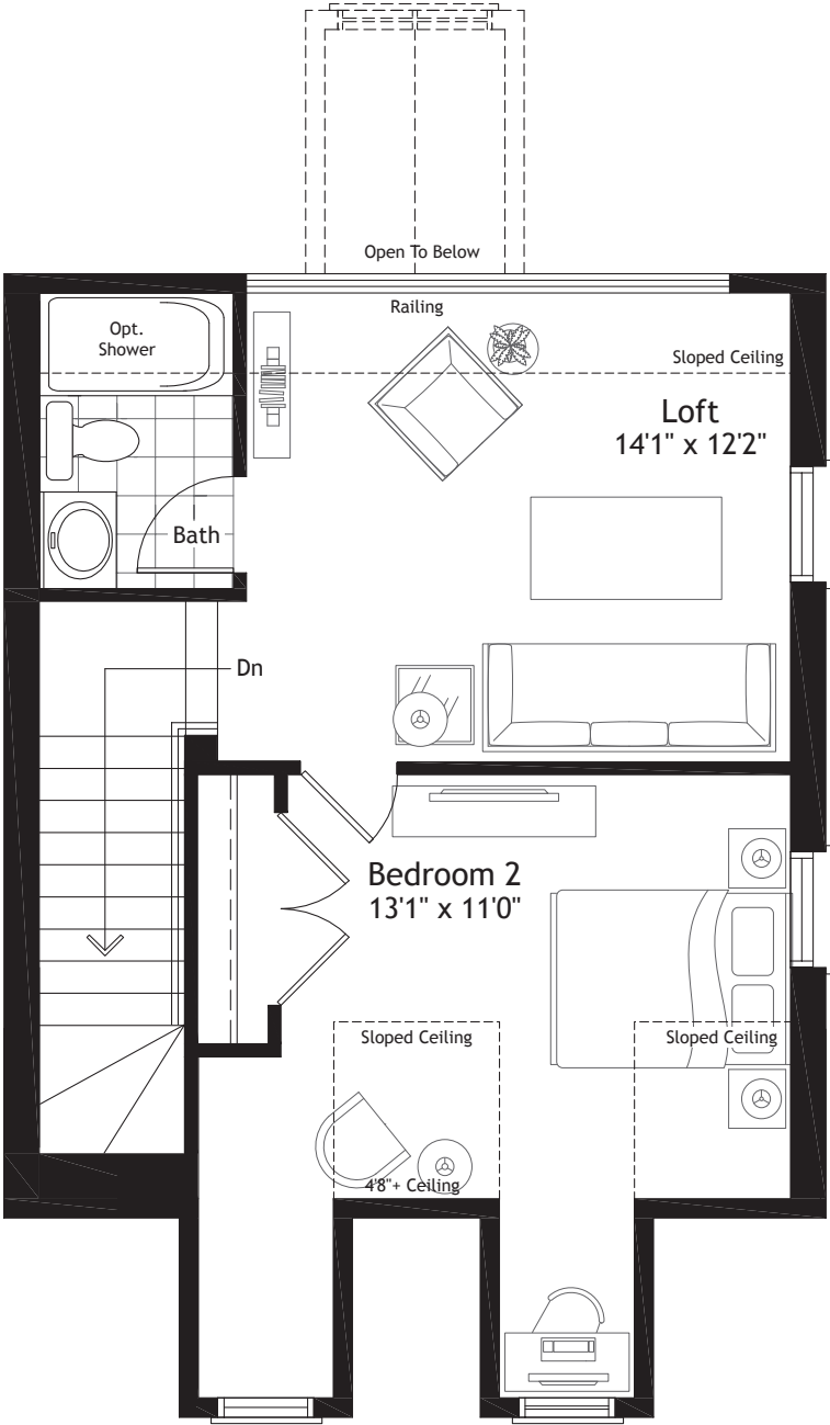
Loft Plan - Elev. C
