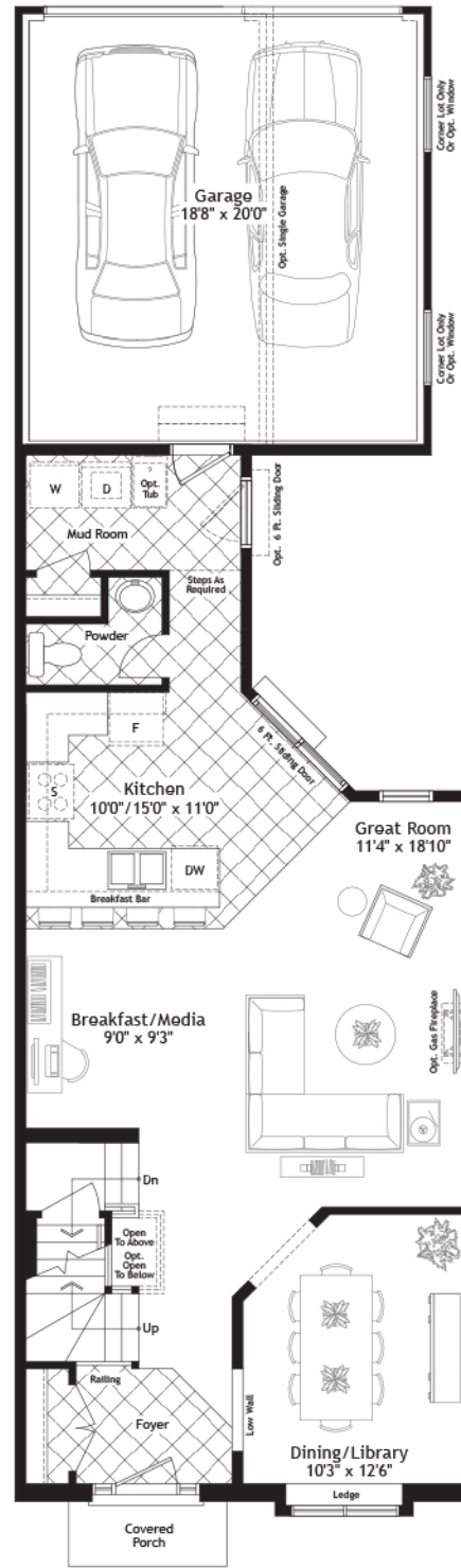
Alt. Main Floor Elev. C
