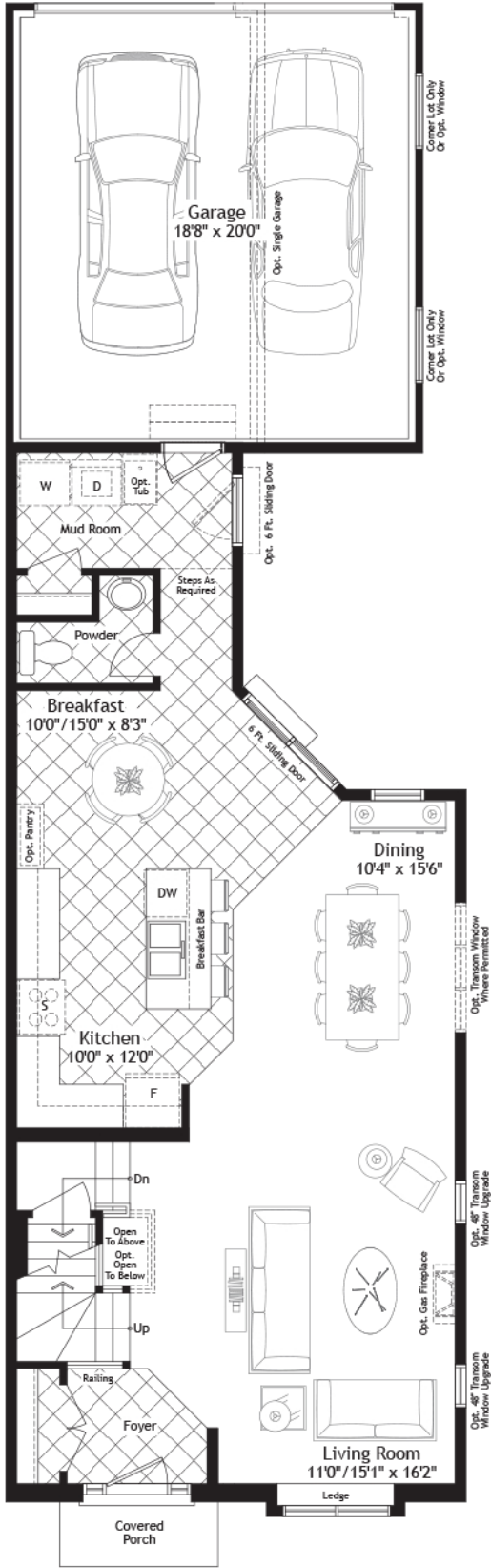
Main Floor Elev. C
