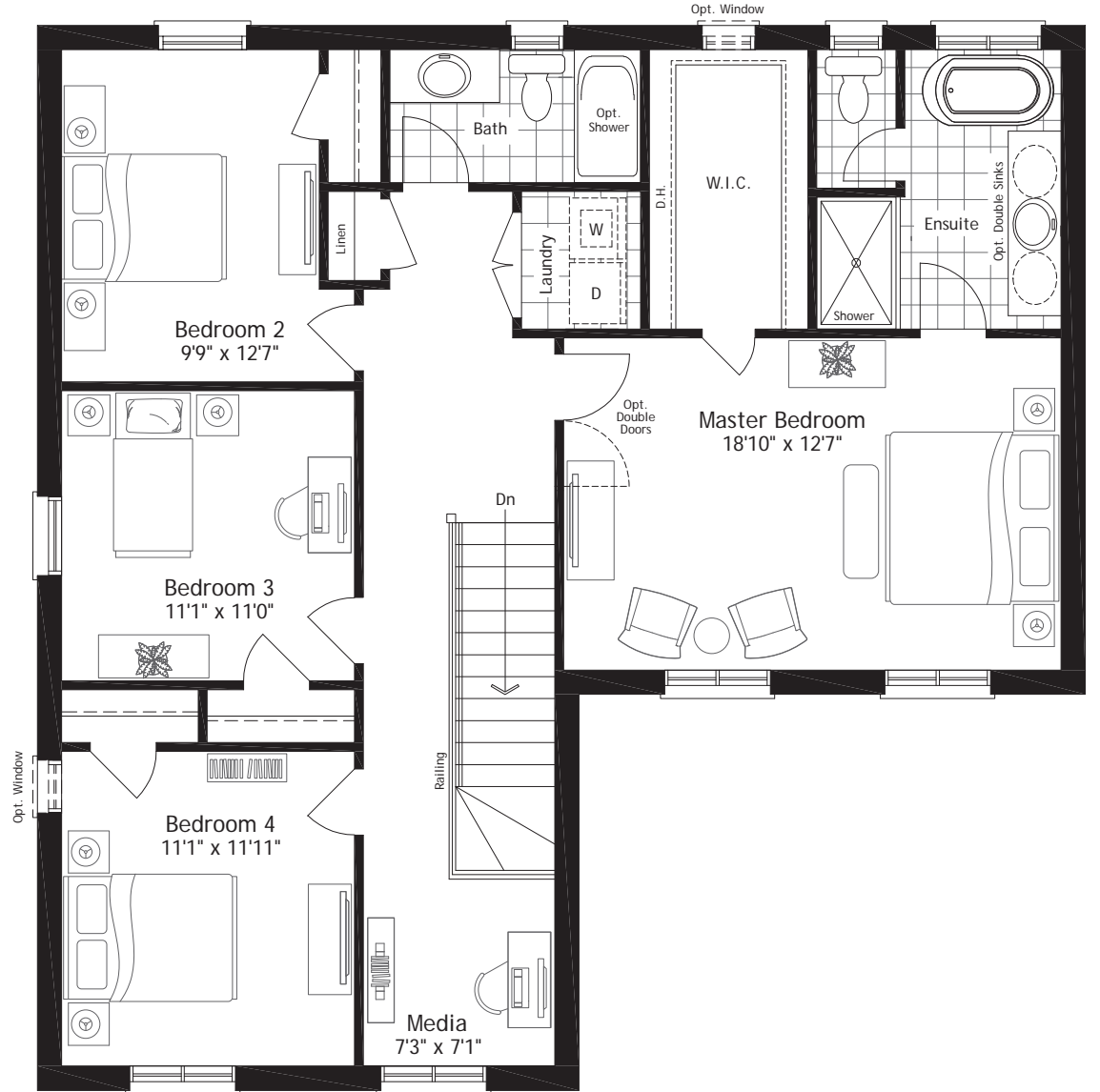
Second Floor Elev. C
