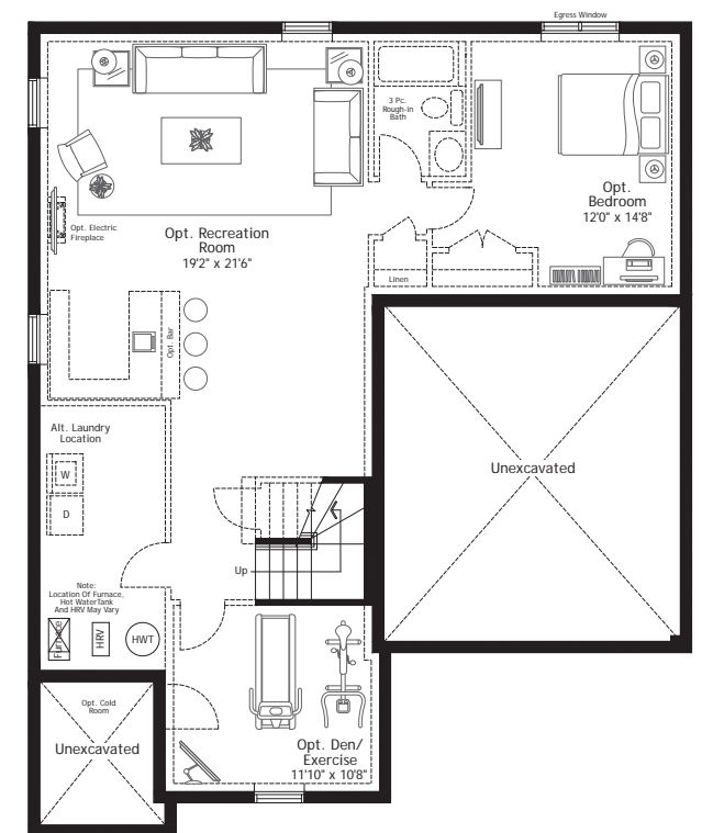
Basement Optional Finished Basement Approx. 1122 sq.ft.
