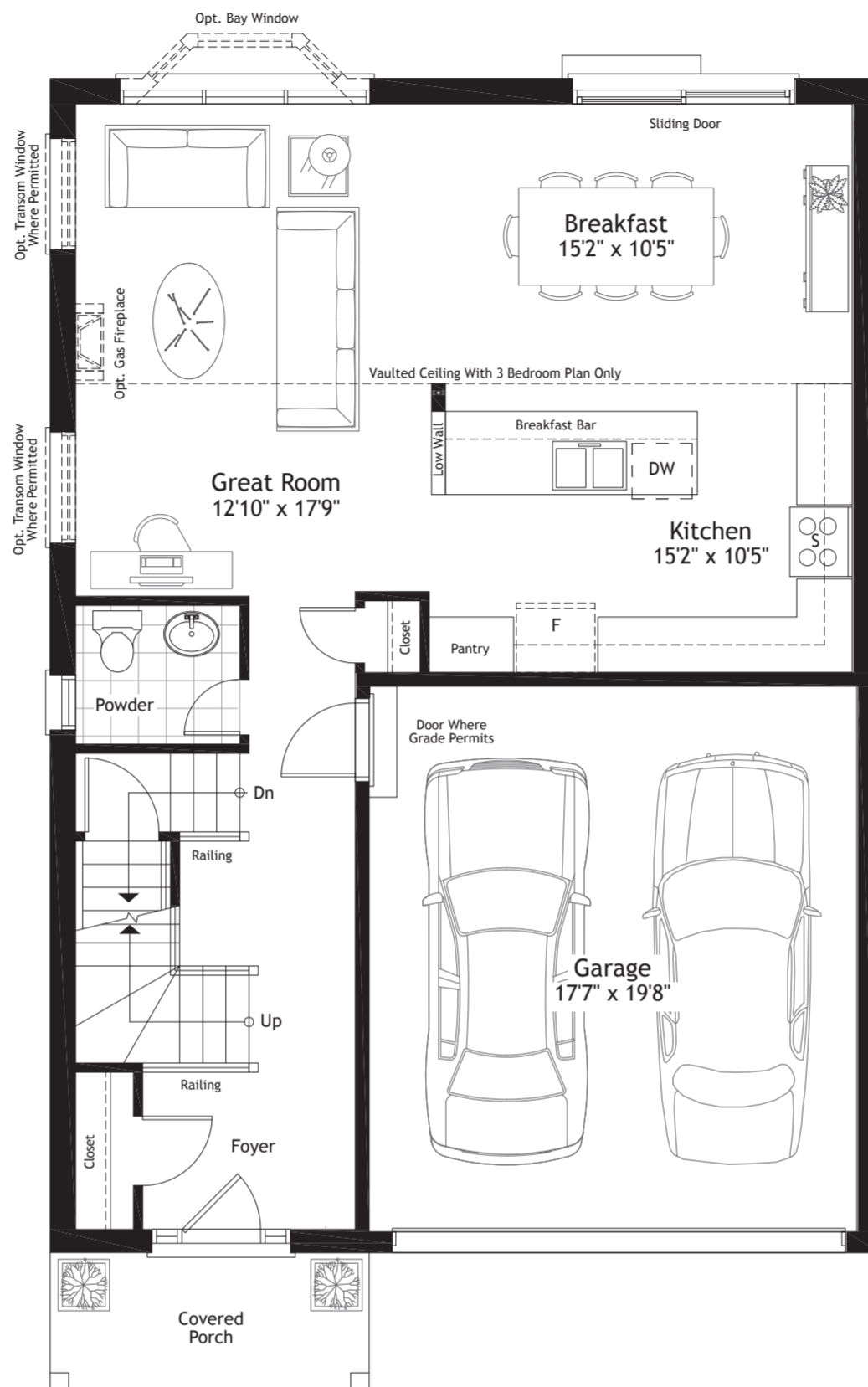
Main Floor
