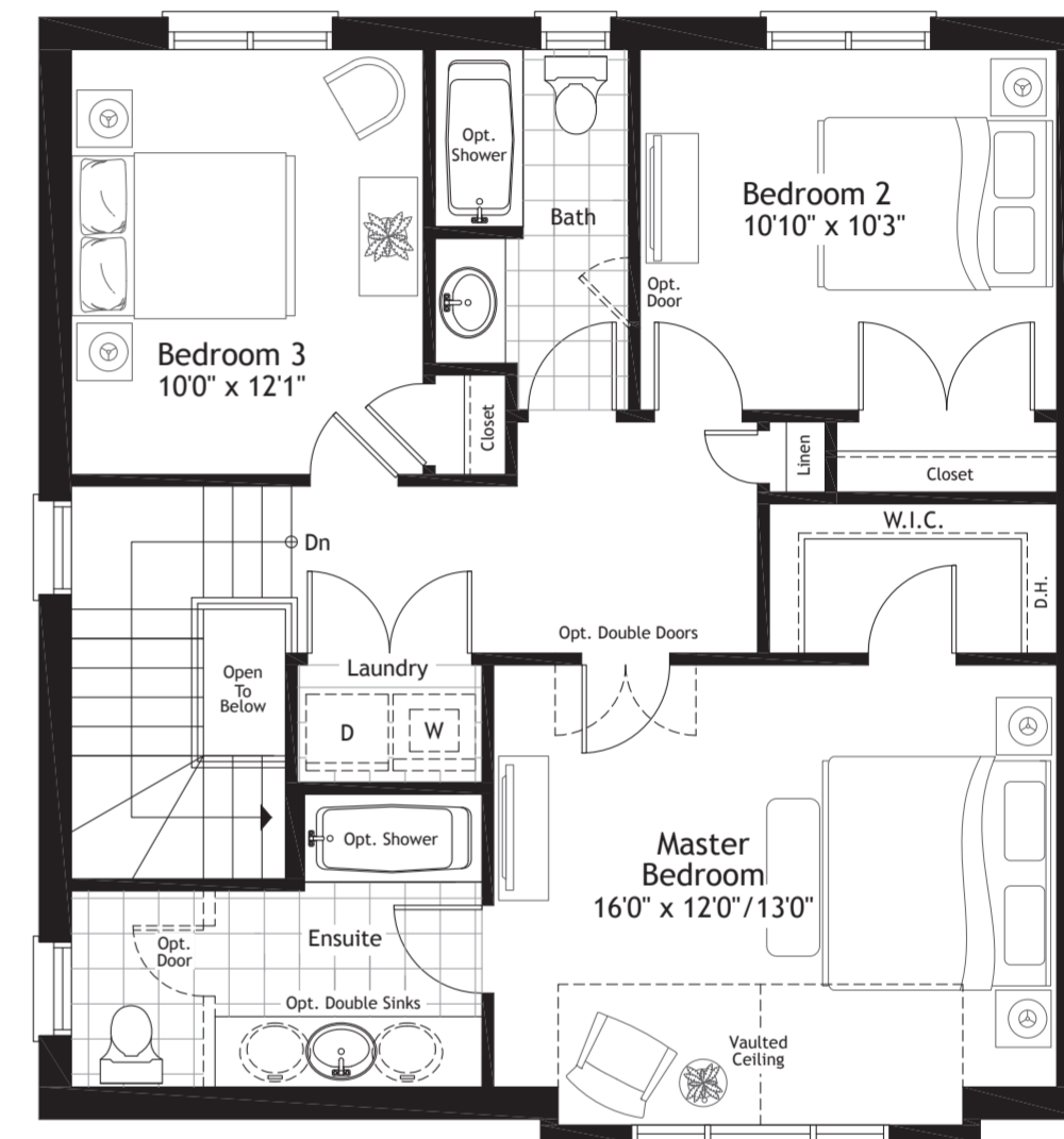
Second Floor 3 Bedroom Plan Elev. C
