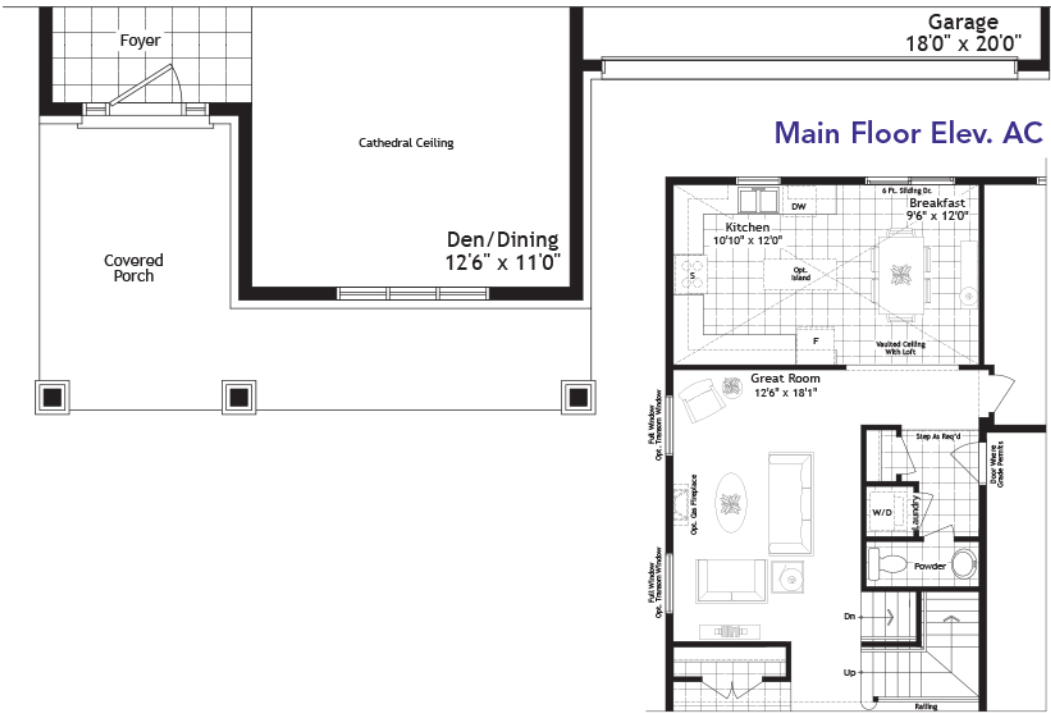
Opt. Main Floor
