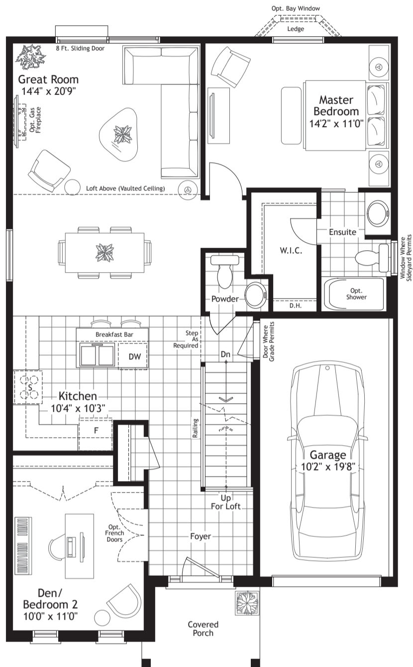
Main Floor Elev. C
