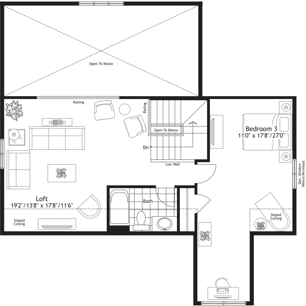
Opt. Loft Plan
