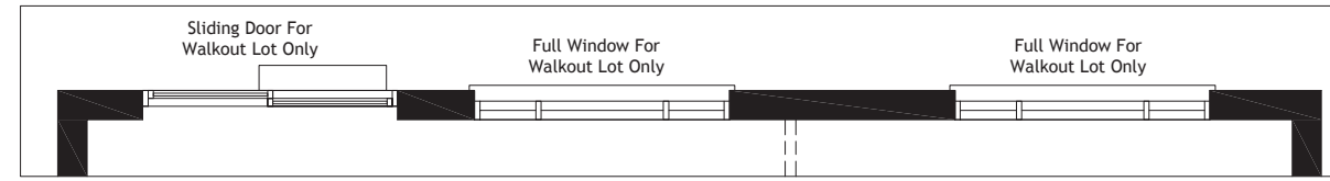
Walkout Basement Layout
