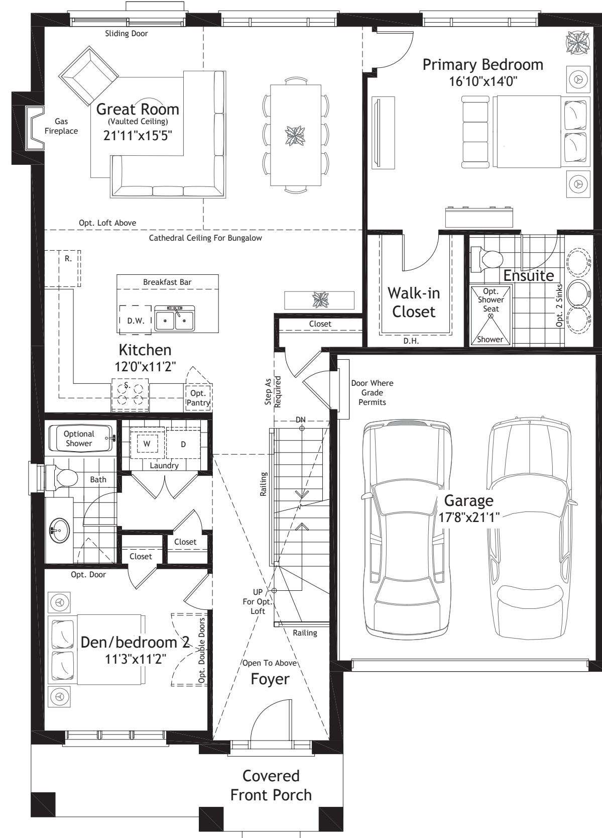
CAMBRAY Elevation 'C' Main Floor Plan - 1507 Sq.ft.
