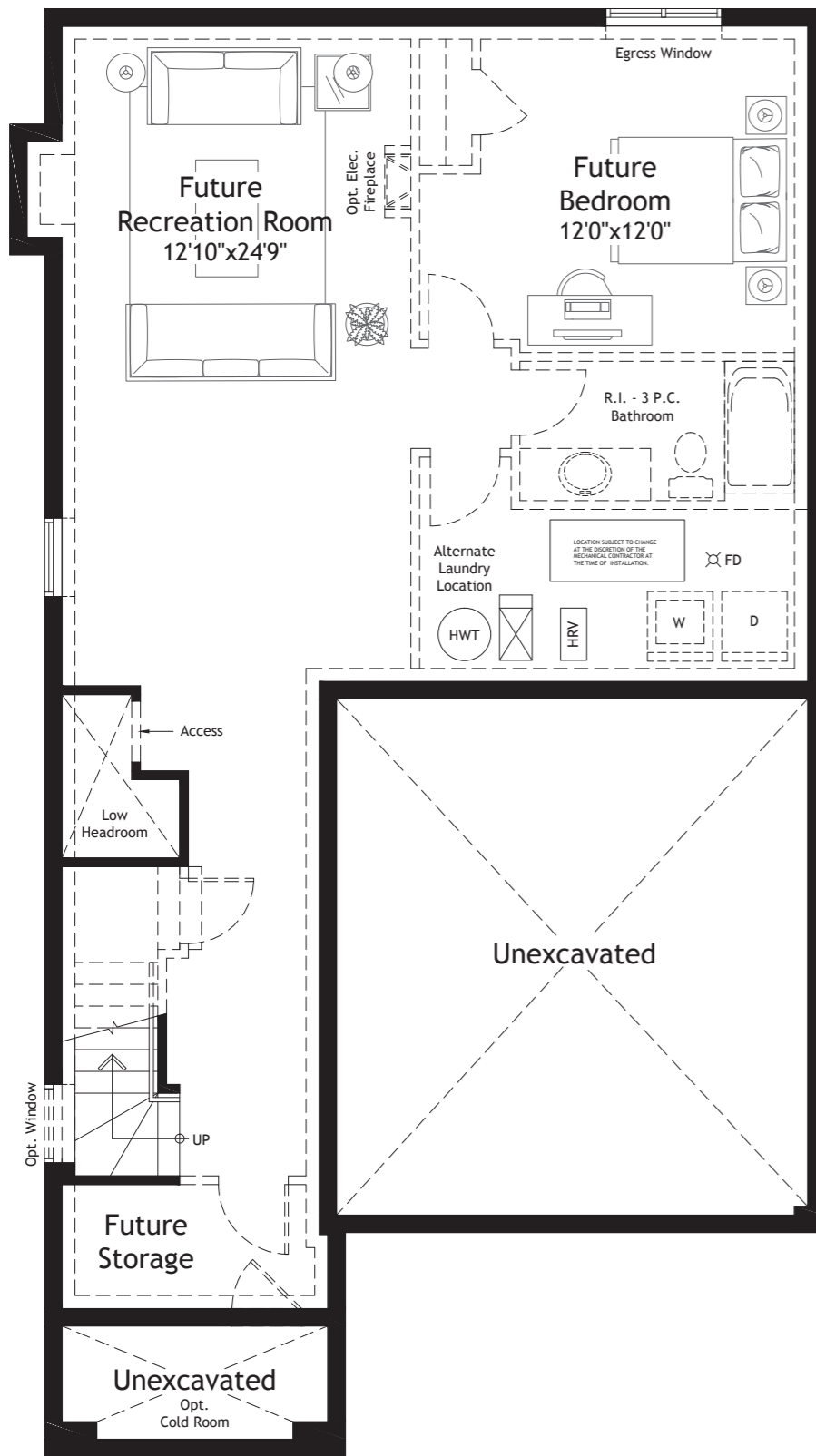
The 'Hartley' Basement Plan - 876 Sq. Ft.
