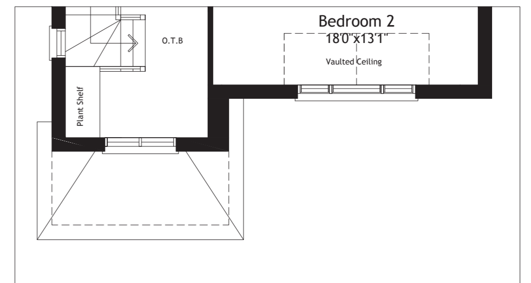
The 'Hartley' Partial Loft Plan Elev. 'AC'
