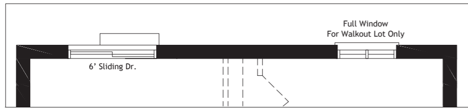
Walkout Basement Layout
