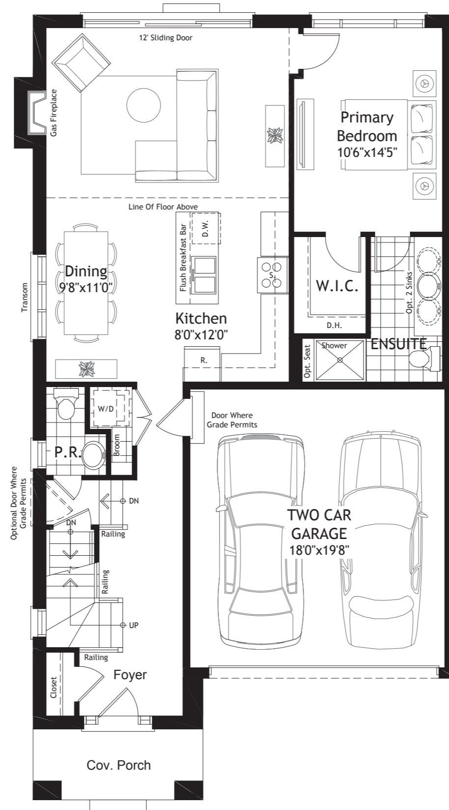
The 'Hartley' Main Floor Plan - 1058 Sq.ft.
