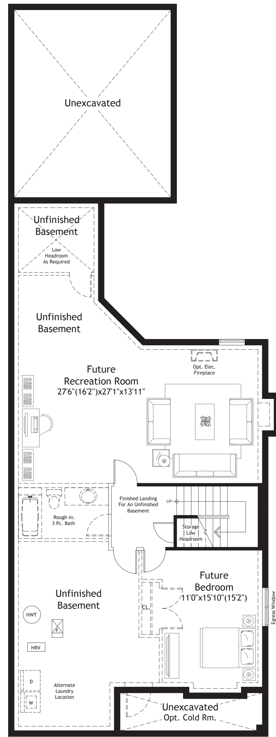
Basement Plan - 896 Sq.ft. Elev. 'C'
