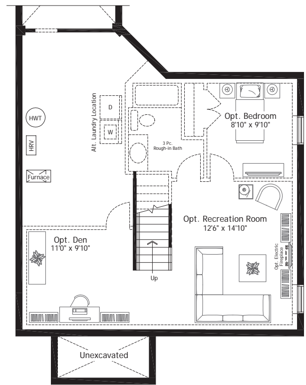
Basement Optional Finished Basement Approx. 632 sq.ft.
