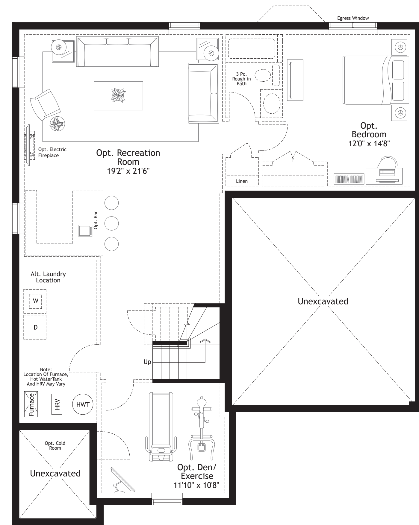
Basement Elev. C
