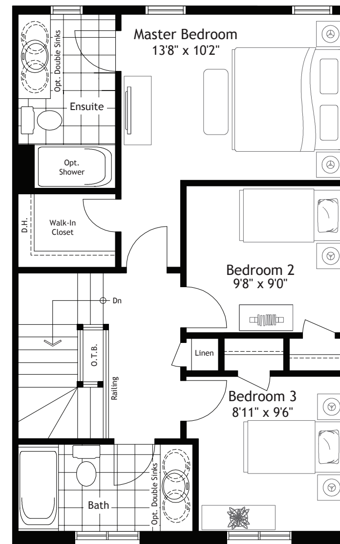
Second Floor - 688 Sq. Ft.
