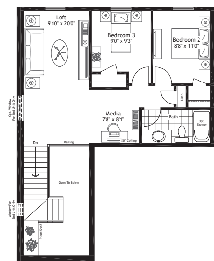
LOFT PLAN OPT. 3 BEDROOM
