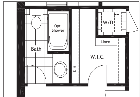
ALT. BATH BLOCKING FOR FUTURE GRAB BARS
