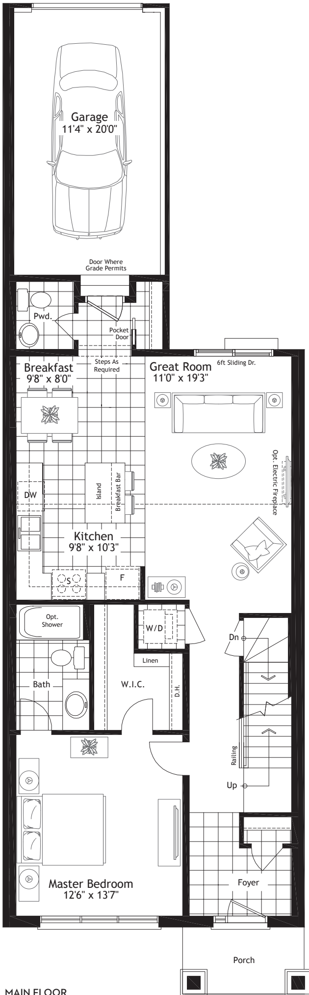
MAIN FLOOR
