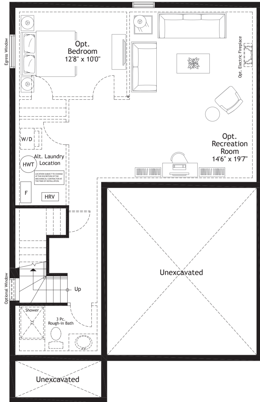
Walkout Basement Layout
