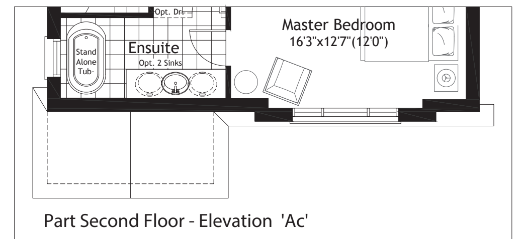
Second Floor - 1270 Sq.ft.
