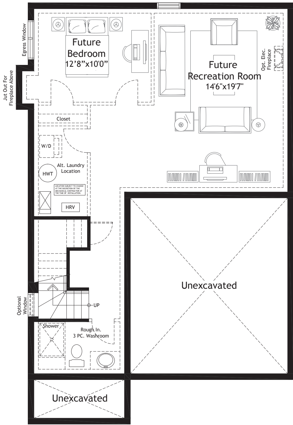
The 'Auburn' Basement Plan - 888 Sq. Ft.
