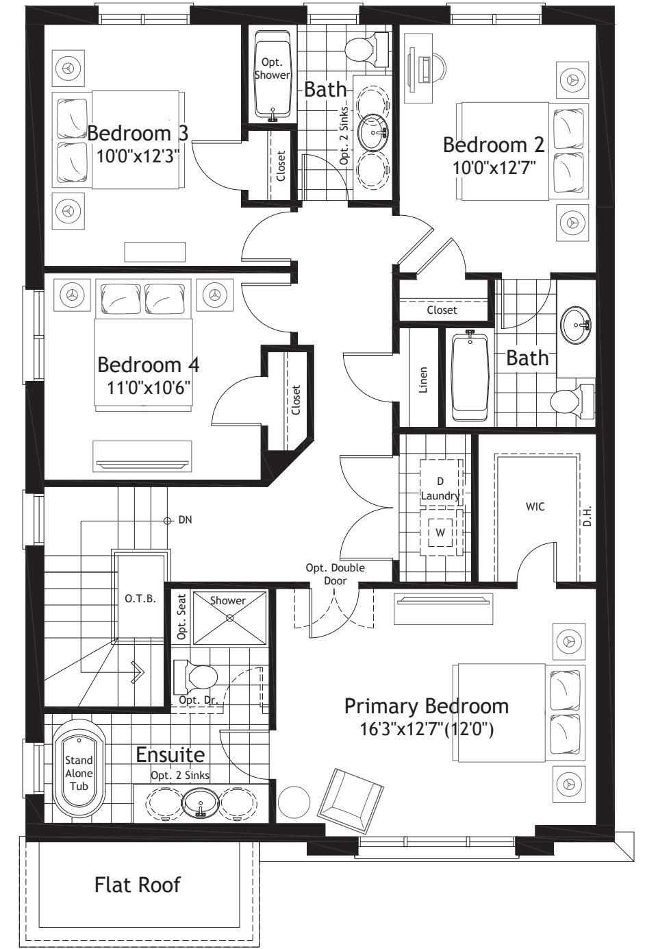
Second Floor - 1270 Sq.ft.
