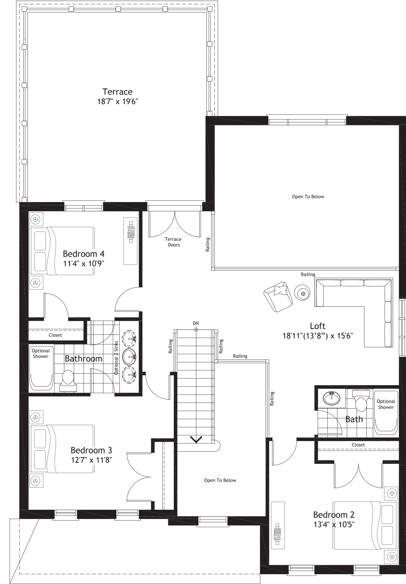
Opt. Loft Plan Elev. C
