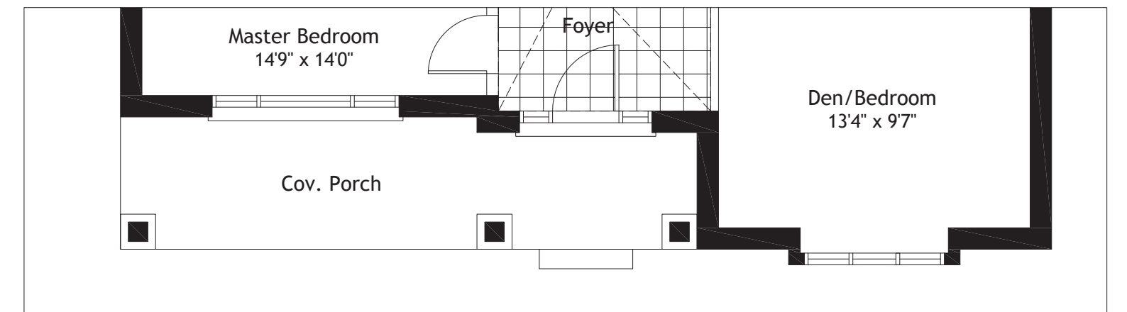
Part. Main Floor Plan Elev. AC
