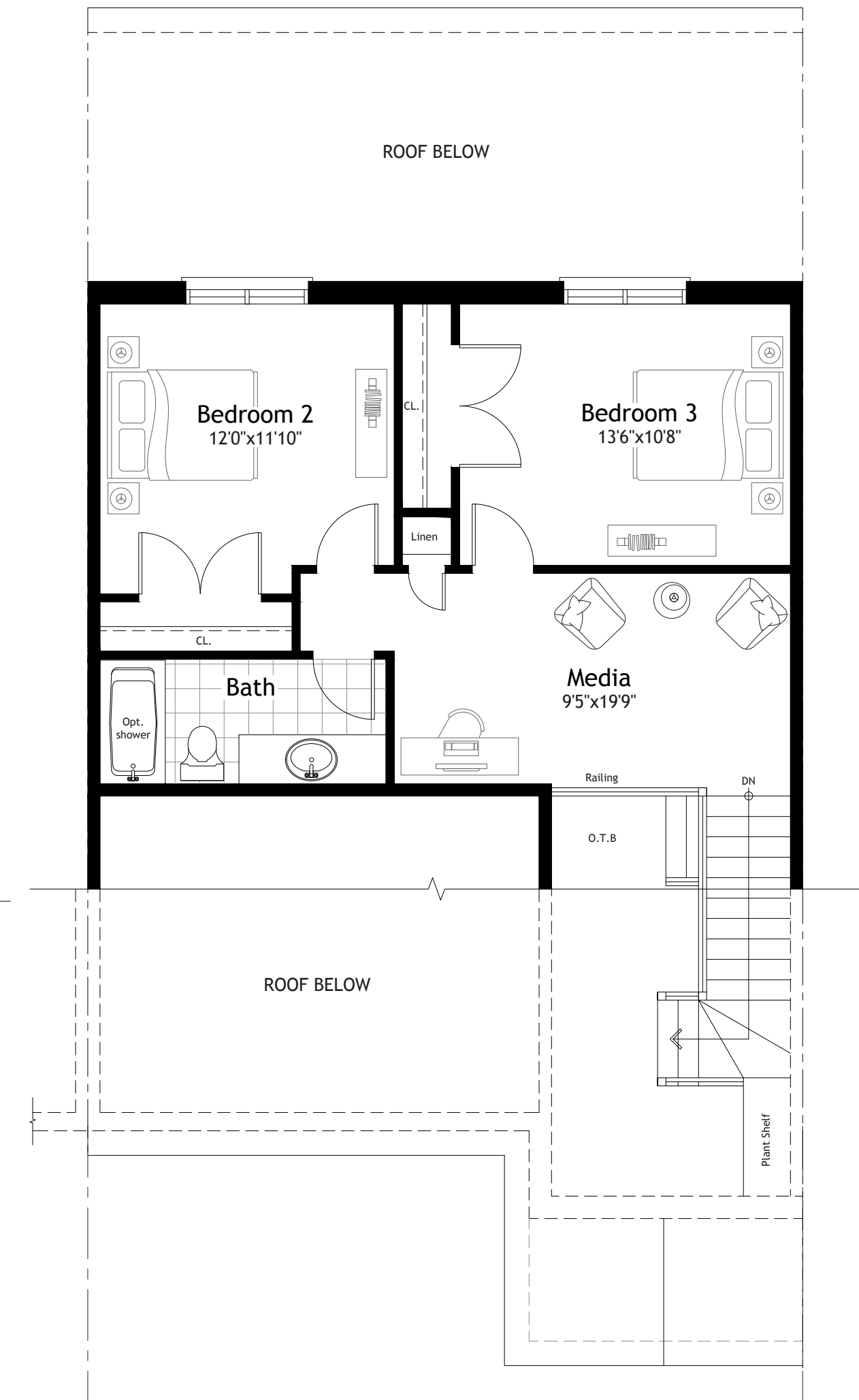
The 'Sinclair' Opt. 3 Bedroom Loft Plan
