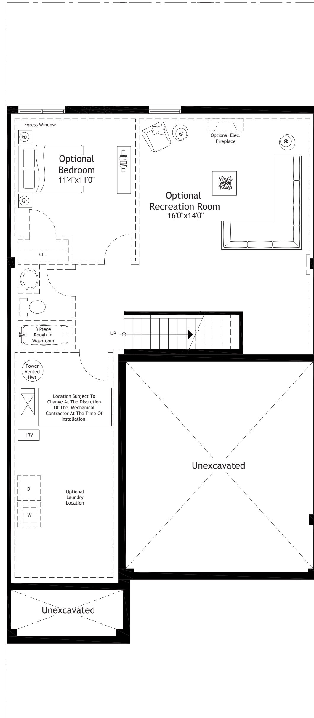
The 'Coverdale' Elev. 'AC' Basement Plan Cobourg Blocks 1,2,3 and 5
